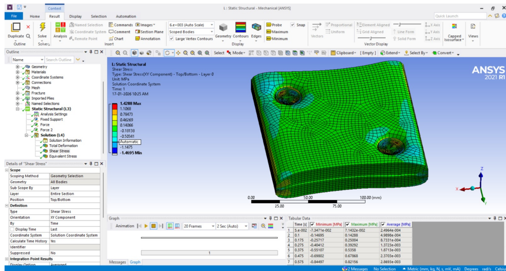
Figure 5.14: Shear Stress 2
