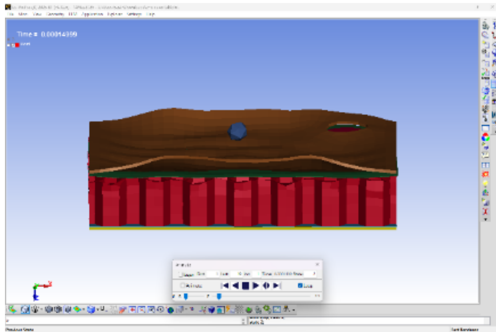
Figure 5.16: Debonding Evolution of single rivert
