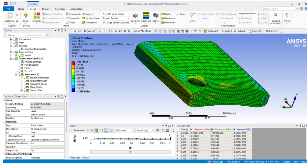
Figure 5.13: Shear Stress 1
