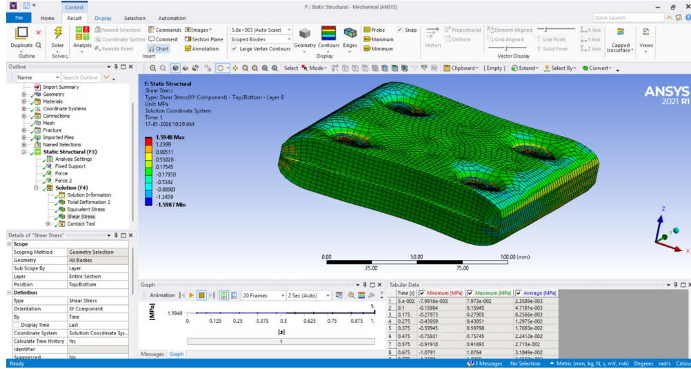
Figure 5.15: Shear Stress 3
